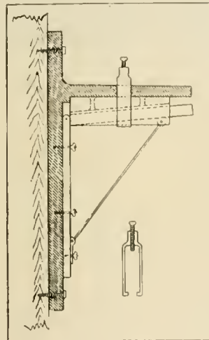
APPLIANCE FOR LINING UP SHOES AND WEDGES.
